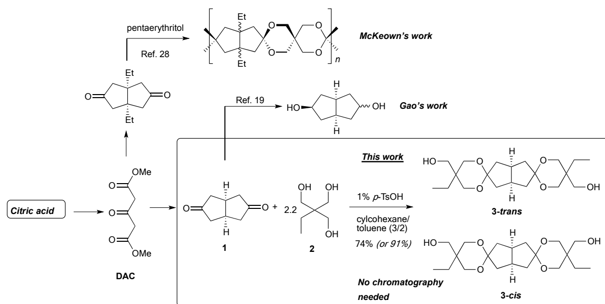
Scheme 1. Outline of the compounds based on diketone 1 reported by McKeown and Gao, and in the present work (inside box). Spiro-diol 3 (mixture of cis and trans ) was synthesized in a ketalization reaction of diketone 1 and a slight excess of TMP 2 (yields of 74 and 91% were obtained when the product was isolated by crystallization and chromatography, respectively).
