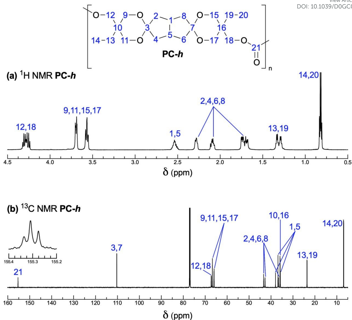
Fig. 3. ^1\text{H} and ^{13}\text{C} spectra of PC- h . ^{13}\text{C} signals indicating the 1:2:1 ratios of cis-cis , cis-trans and trans-trans dyads are shown separately in the carbonyl region.
