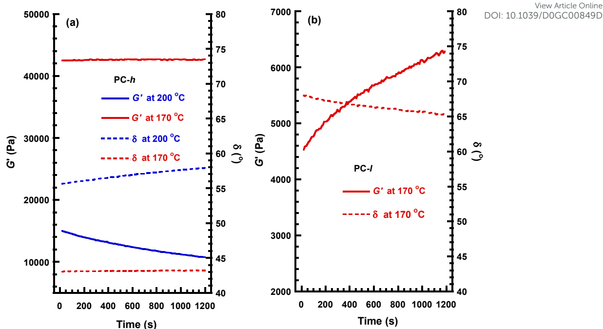
Fig. 8. Variation of the melt shear storage modulus ( G' ) and phase shift ( \delta ) during time sweeps of PC-h at 170 and 200 °C (a) and PC-l at 170 °C (b), as measured by rheology at 1 Hz, 0.2% strain (note the different scales for G' ).
