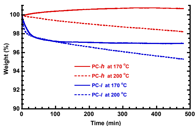
Fig. 6. Isothermal TGA measurements of PC- l and - h at 170 and 200 °C.
