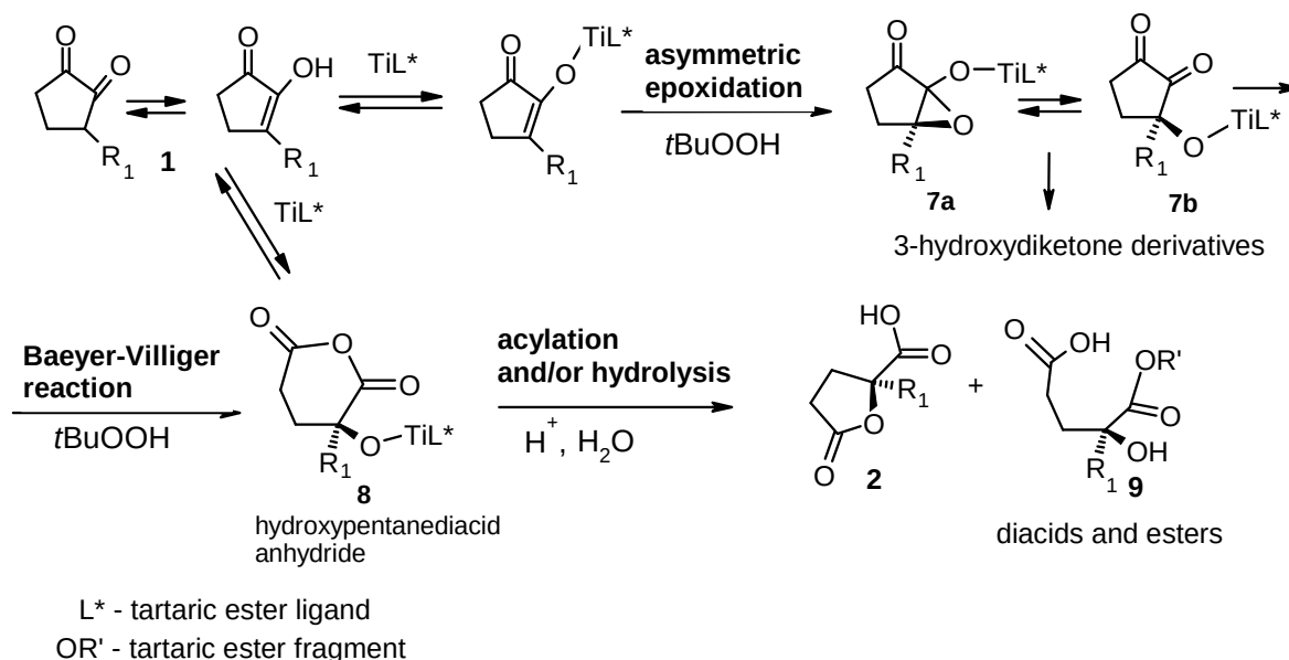
Scheme 3. The formal reaction cascade
