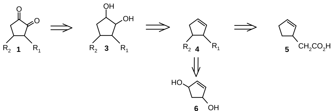
Scheme 2. Retrosynthetic sequence for 3-substituted 1,2-cyclopentanediones 1 .
