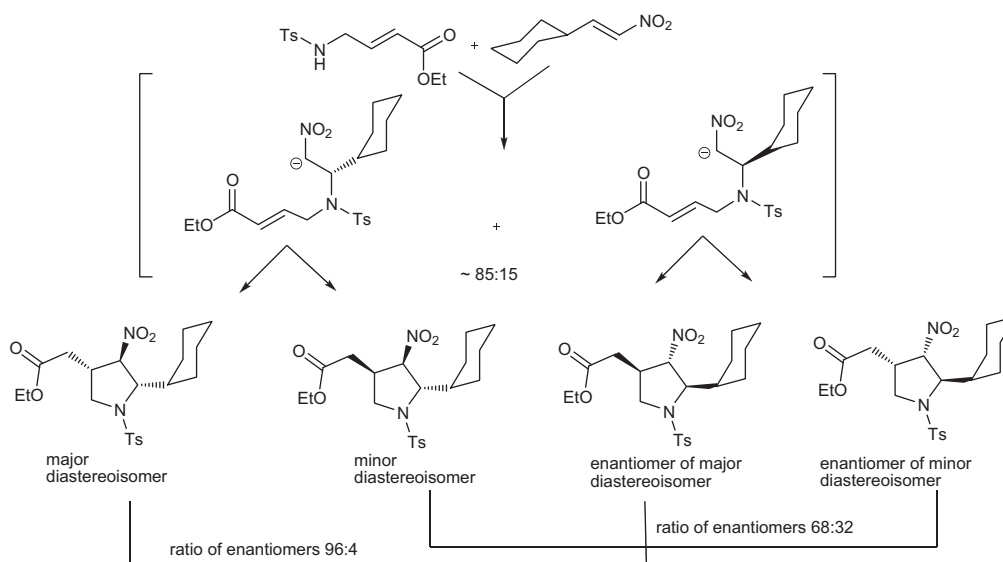
Scheme 6. Distribution of the stereoisomers in the formation of pyrrolidines 4g and 4g' .
