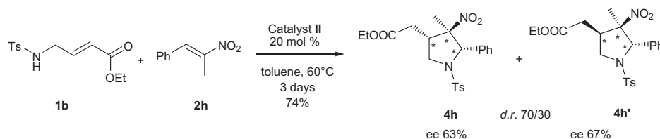
Scheme 2. Reaction with ( E )-β-methyl- trans -β-nitrostyrene.
