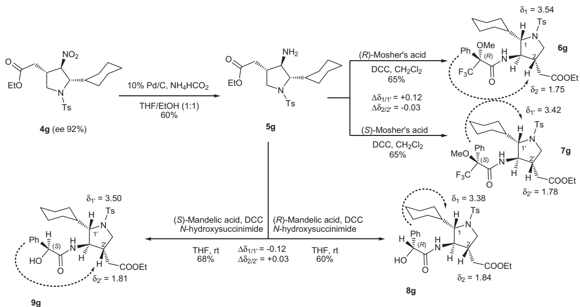
Scheme 3. Determination of the absolute configuration of pyrrolidine 4g .
