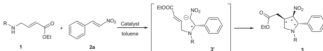
Scheme 1. Synthesis of trisubstituted chiral pyrrolidines.
