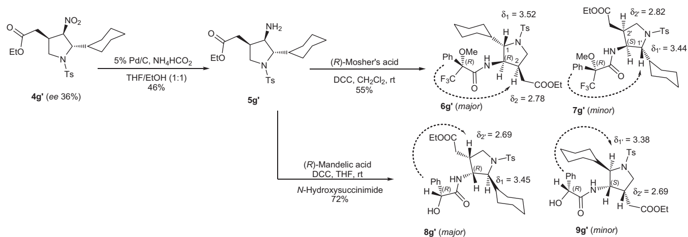
Scheme 4. Determination of the absolute configuration of pyrrolidine 4g' .
