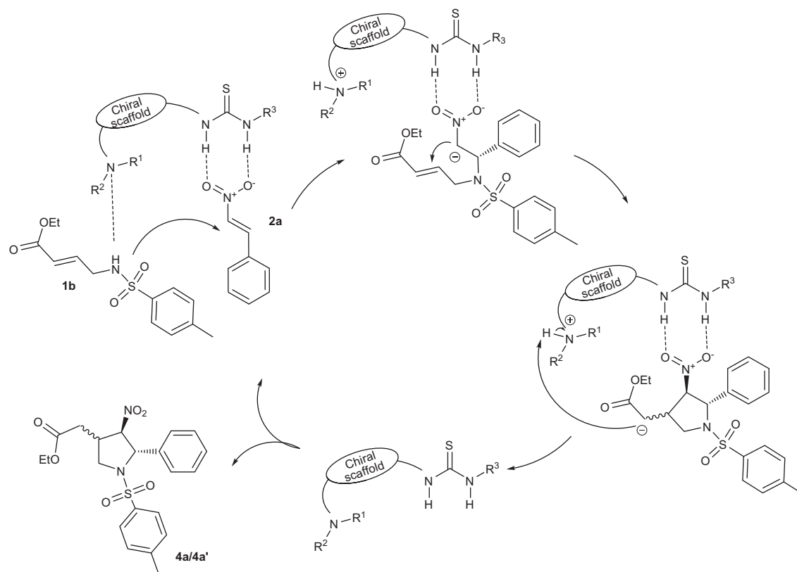
Scheme 5. Proposed mechanism of the thiourea catalyzed formation of chiral substituted pyrrolidines.
