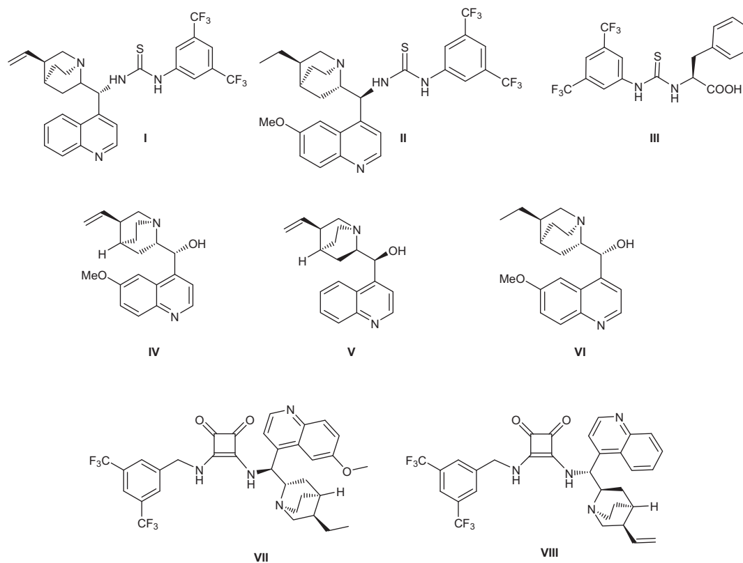
Figure 1. Catalysts used in the synthesis of chiral pyrrolidines.
