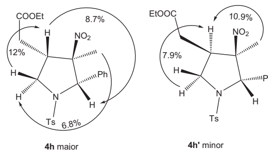
Figure 2. NOE results of pyrrolidines 4h and 4h' .
