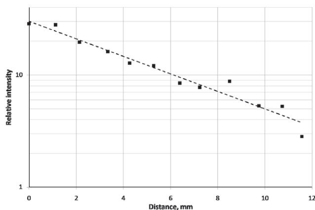
Figure 13. Attenuation of 532 nm laser light propagating within a sol-gel-prepared \text{ZrO}_2 fibre of 3\text{ }\mu\text{m} diameter. The fit (dashed line) corresponds to a loss of 0.8\text{ dB mm}^{-1} .
