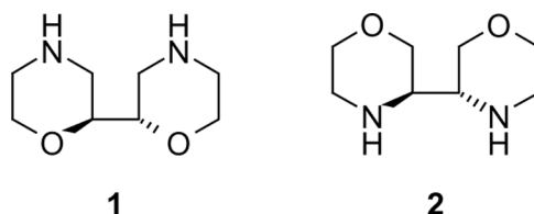
Figure 1. 2,2'-Bimorpholine 1 and 3,3'-bimorpholine 2 .
