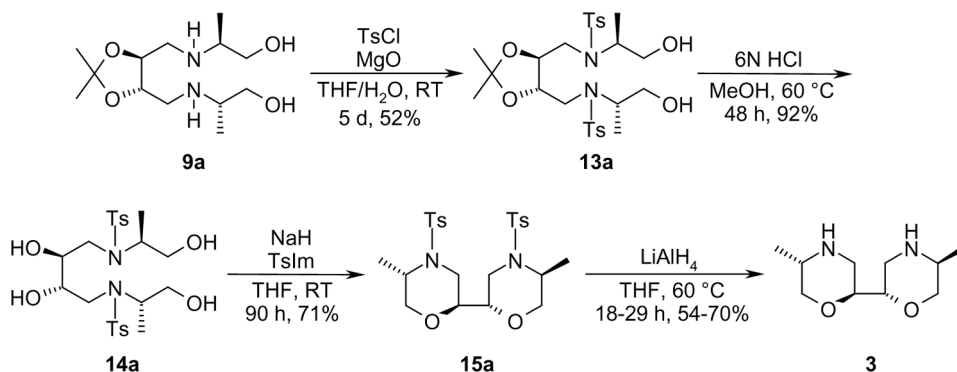
Scheme 2. Synthesis of bimorpholine 3.
