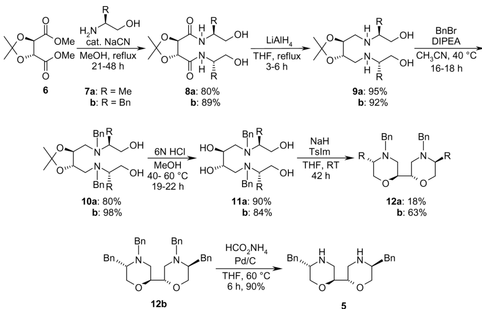
Scheme 1. Synthesis of bimorpholine 5 .
