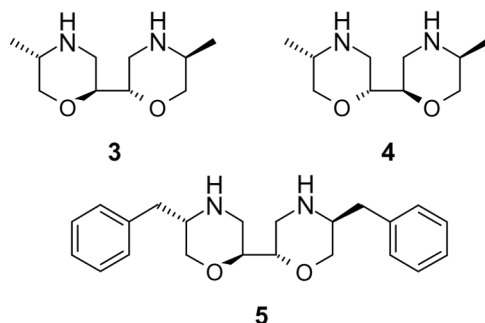
Figure 2. 5,5'-Disubstituted bimorpholines.
