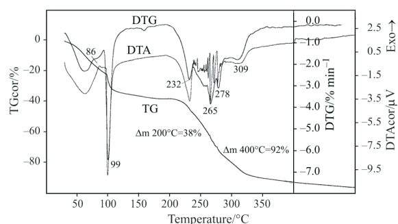
Fig. 1 TG, DTG, DTA curves of UF3 curing with 2% \text{NH}_4\text{Cl}
