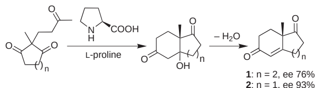
Scheme 1 Proline-catalyzed synthesis of Wieland–Miescher ketone (1) and its nor-analogue 2
