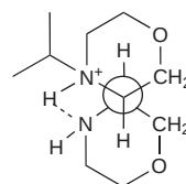
Figure 2 Proposed hydrogen-bonded structure of the bismorpholine–acid catalyst
