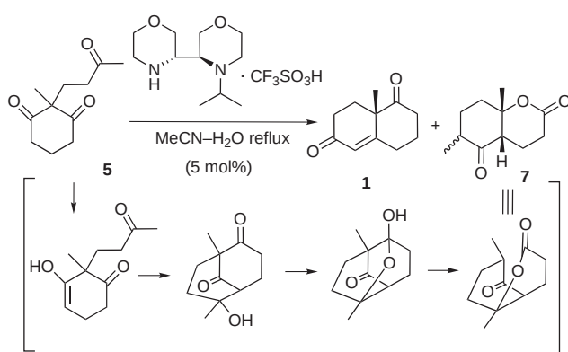
Scheme 2 Formation of side-product 7
