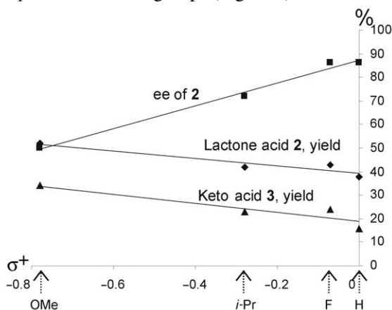
Figure 1 Correlation of yields of \gamma -lactone acids 2a–d , keto acids 3a–d and enantiopurity of 2a–d with \sigma^+ constants of the para substituents. 8
