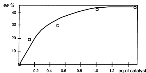
Figure 2. Dependence of the enantioselectivity of oxidation of cyclobutanone 1a on the amount of reagent A
