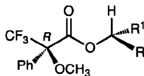
(A) R -MTPA ester
