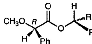
(B) R -MPA ester
